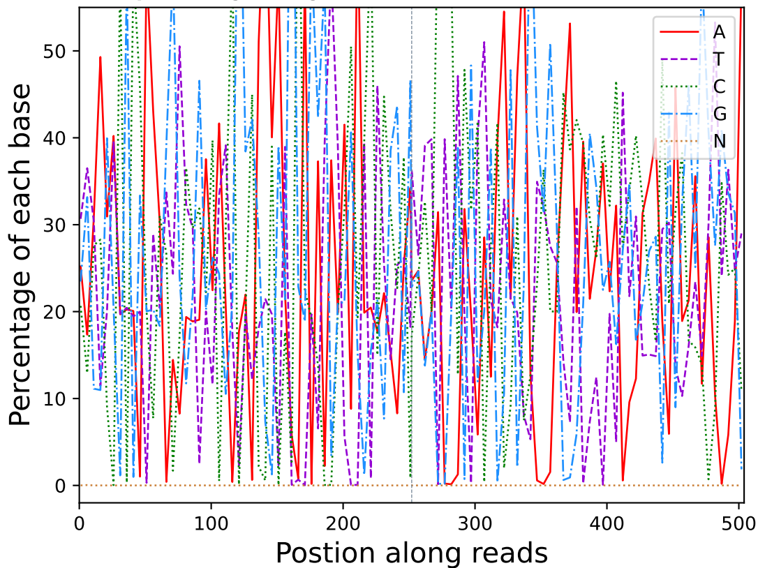
Base percentage along reads (R10222)
